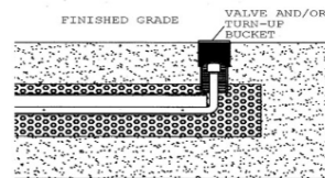
Low Pressure Pipe System
