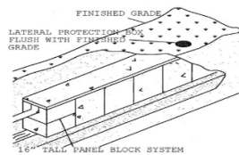
Panel Block System
